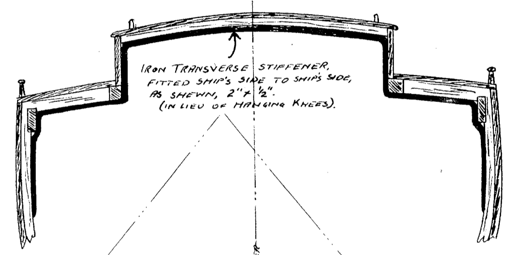
SKETCH OF TRANSVERSE STIFFENER.
